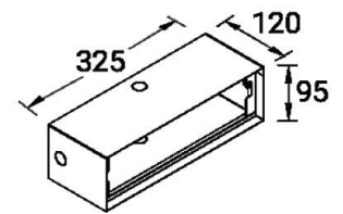
RECESSING BOX
