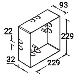
RECESSING BOX
