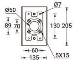
Mounting detail
