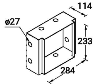
RECESSING BOX
